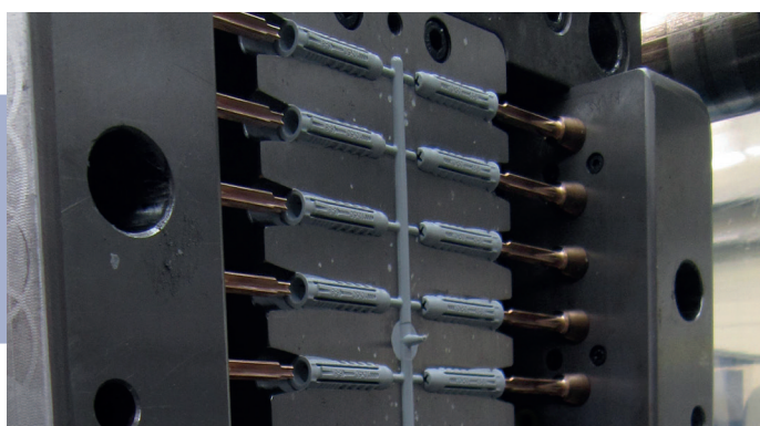
INJECTION DE NYLON
